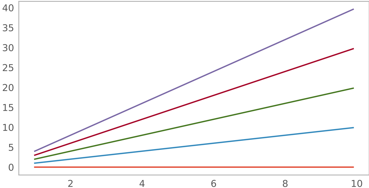
Polynomial1D with a 5 model set on the same input
