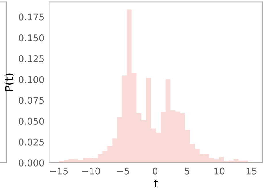
hist(t, bins="freedman")
