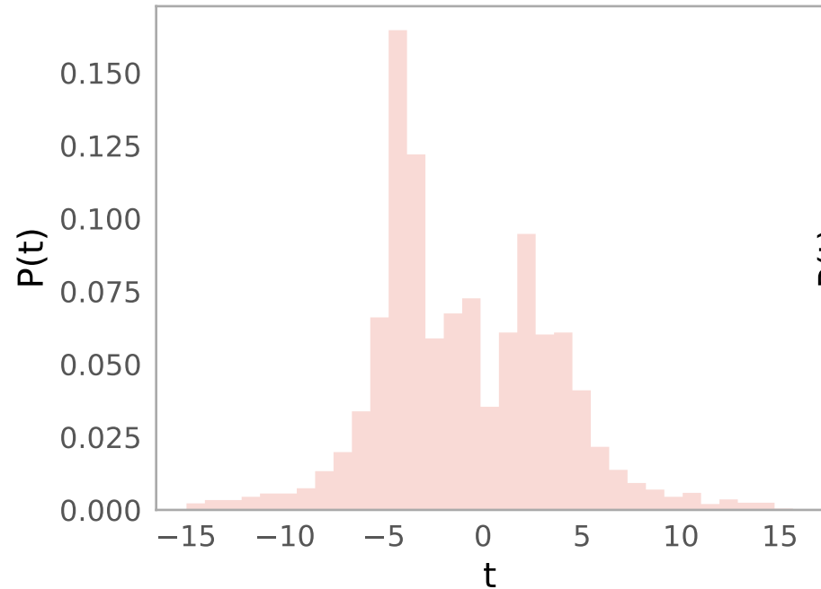
hist(t, bins="scott")
