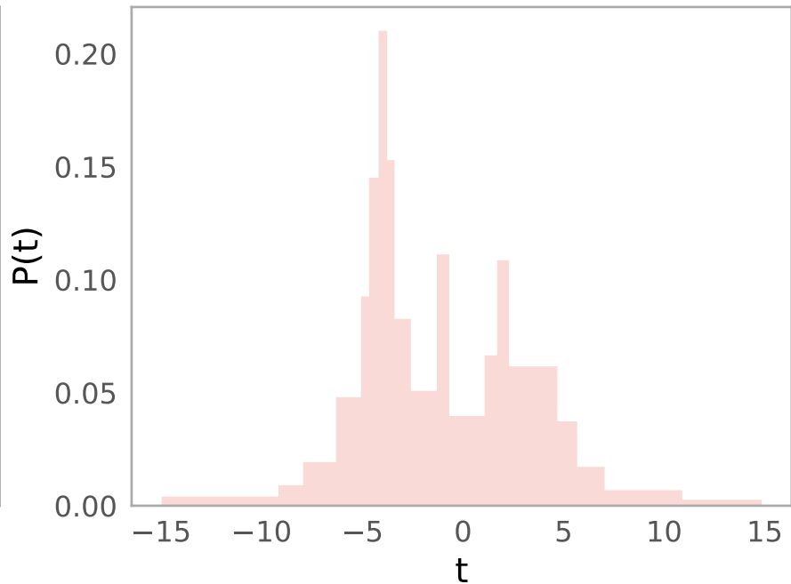
hist(t, bins="blocks")
