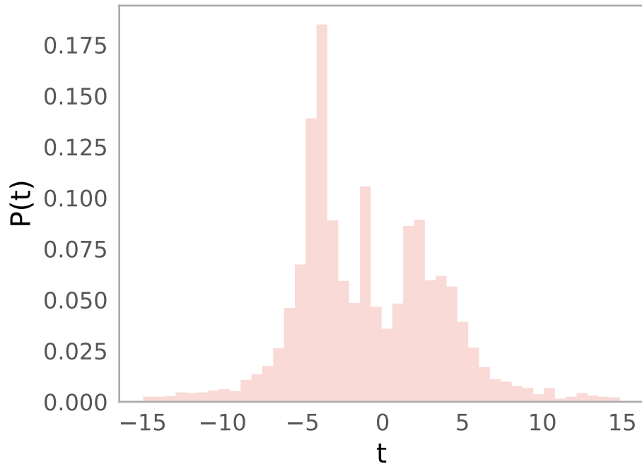
hist(t, bins="knuth")
